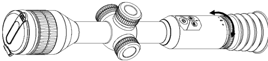
Figure 3-1 Adjust Diopter
